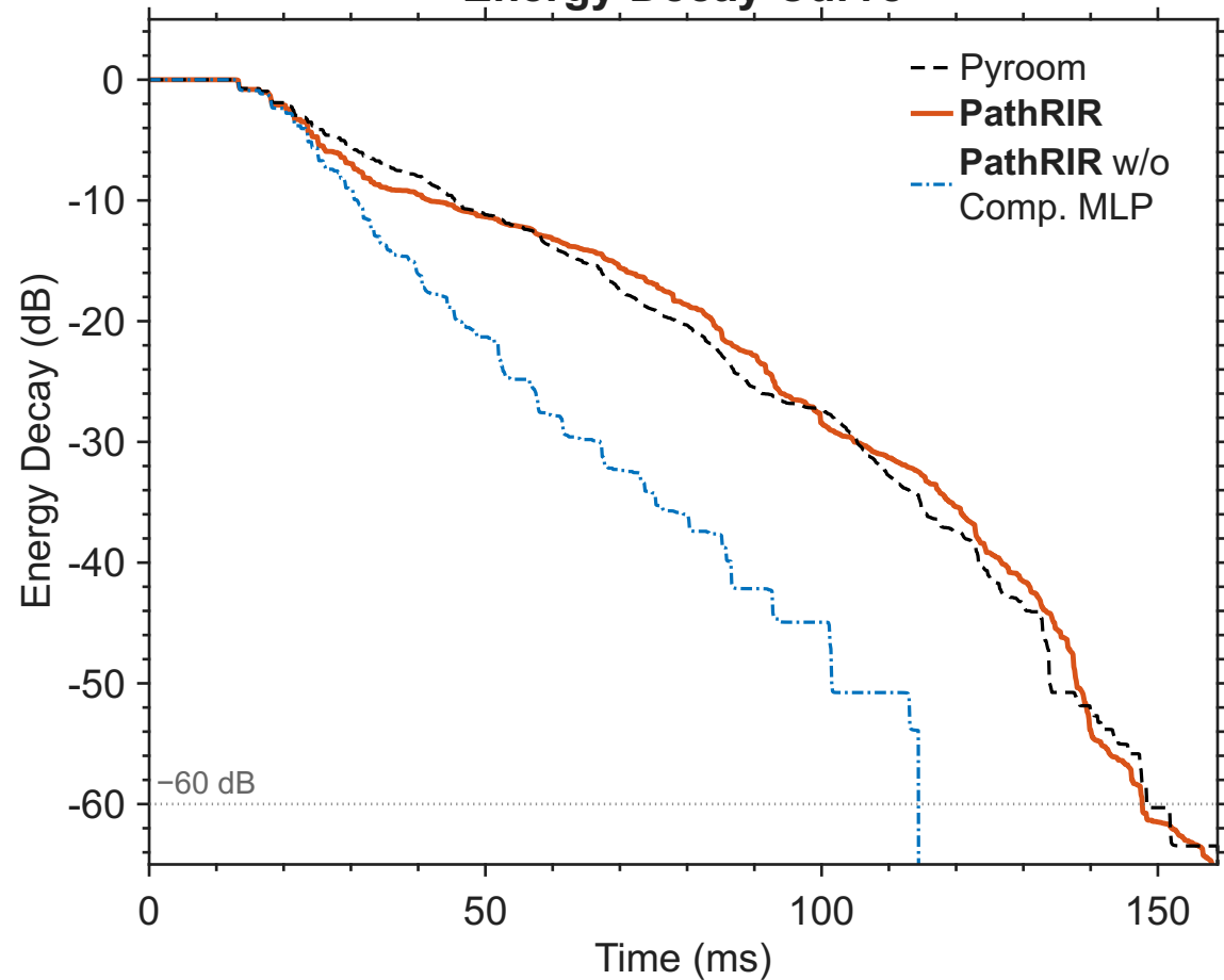
Energy Decay Curve
